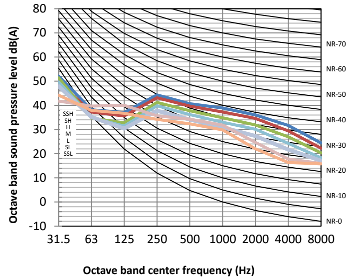
MHG-48HAN1 octave band levels
