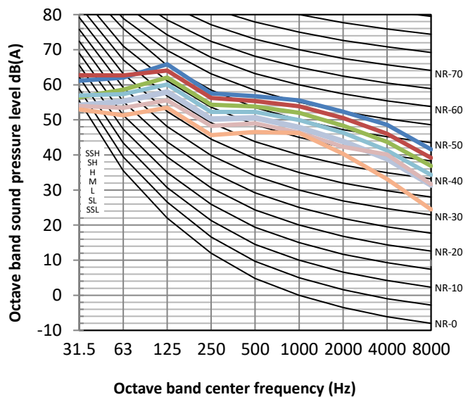
MHG-192HAN1 octave band levels
