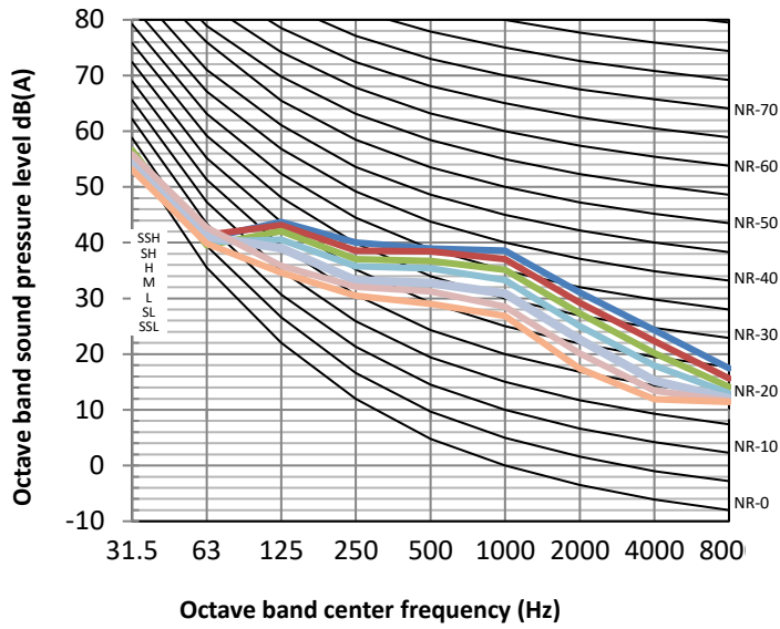
MHG-28HAN1 octave band levels
