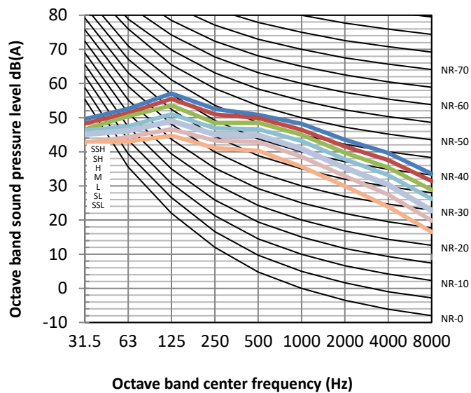
MHG-120HAN1 octave band levels
