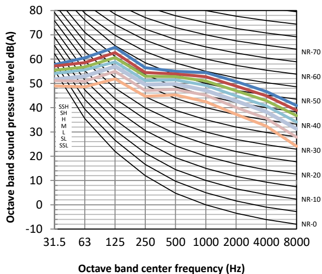
MHG-140HAN1 octave band levels
